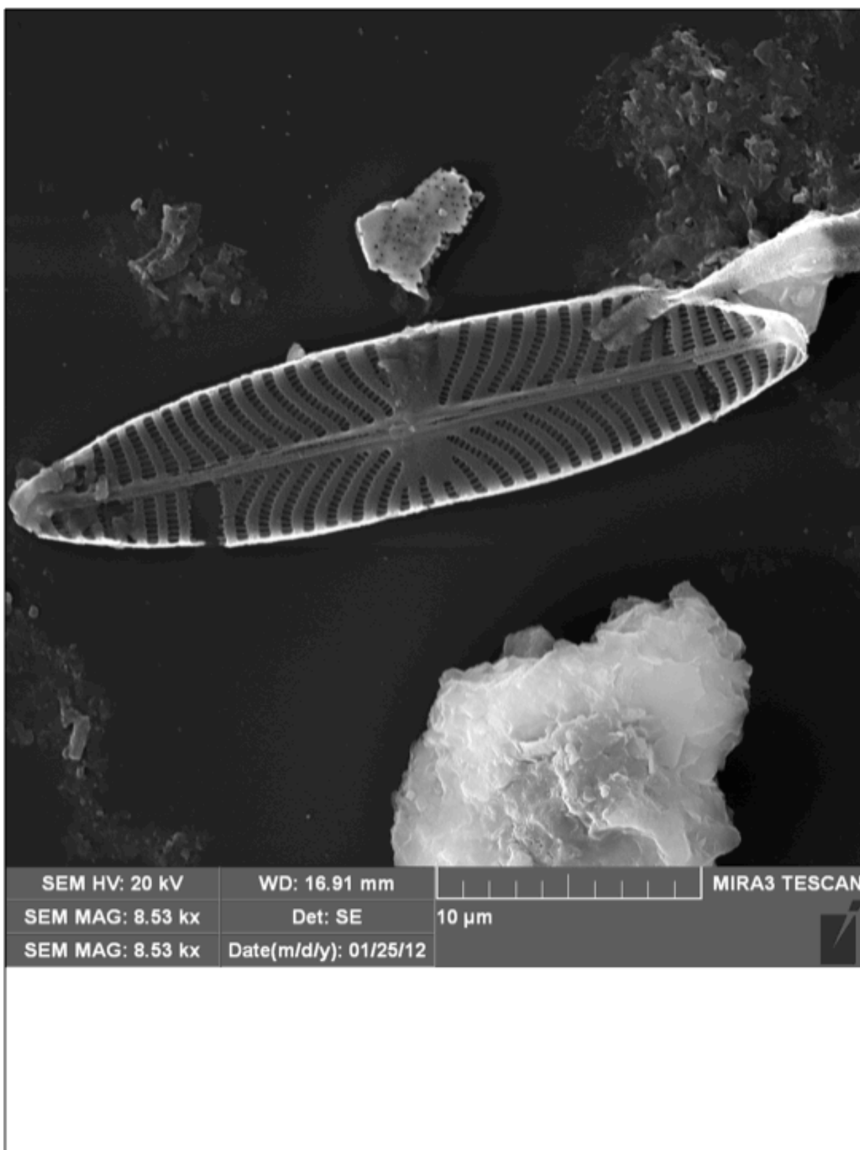
Figure A1.126: SEM identification plate for: Navicula cari
