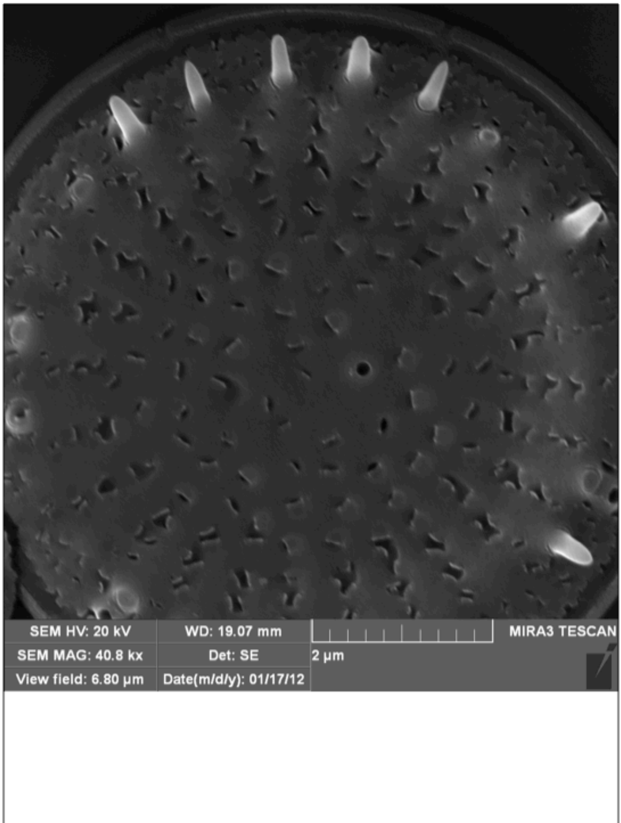
Figure A1.62: SEM identification plate for Stephanodiscus minutulus
