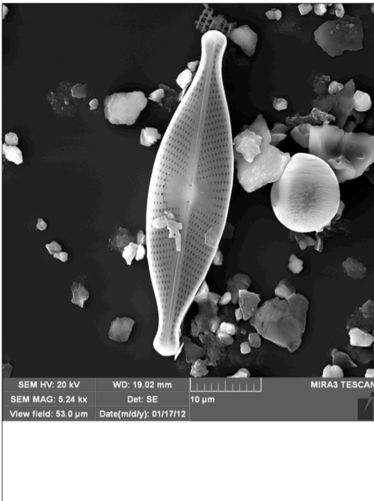
Figure A1.134: SEM identification plate for: Navicula rhynchocephala
