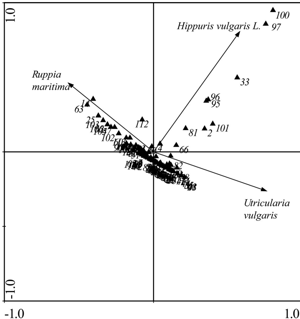
Figure A2.7: CCA ordination diagram of diatoms and macrophytes, including significant macrophyte species and all diatom species, with macrophytes included in analysis as environmental variables.
