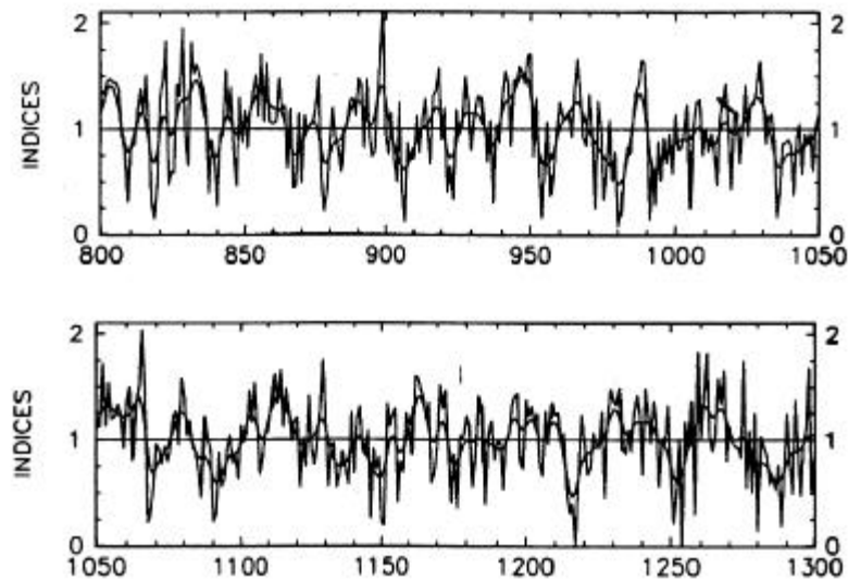
Figure 4.2 - Standardized tree-ring index (Fritts and Dean 1992: 54).
